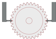
GEAR TOOTH OUTSIDE CONTROLLO DENTATURE ESTERNE
