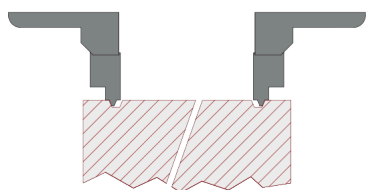
DIAMETER ORING 23° CONTROLLO DIAMETRI ORING 23°
